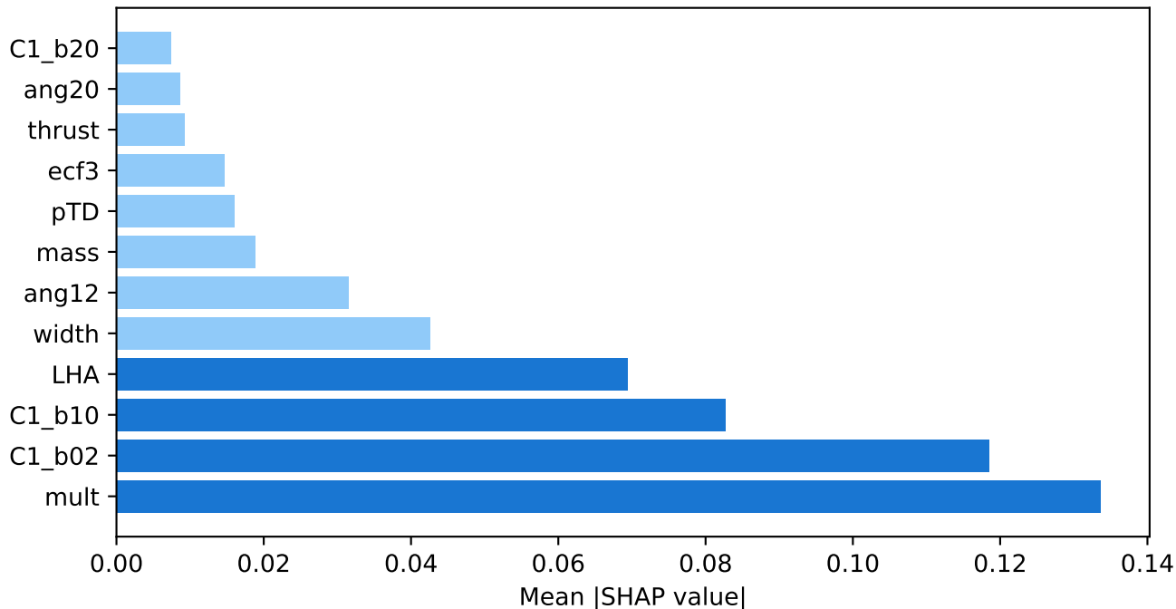
SHAP Feature Importance -- MAE-pretrained
