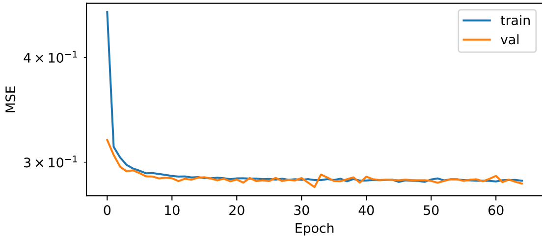
MAE Pre-training
