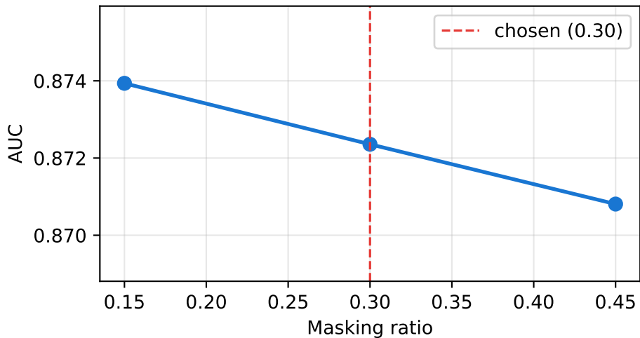
Ablation: mask ratio
