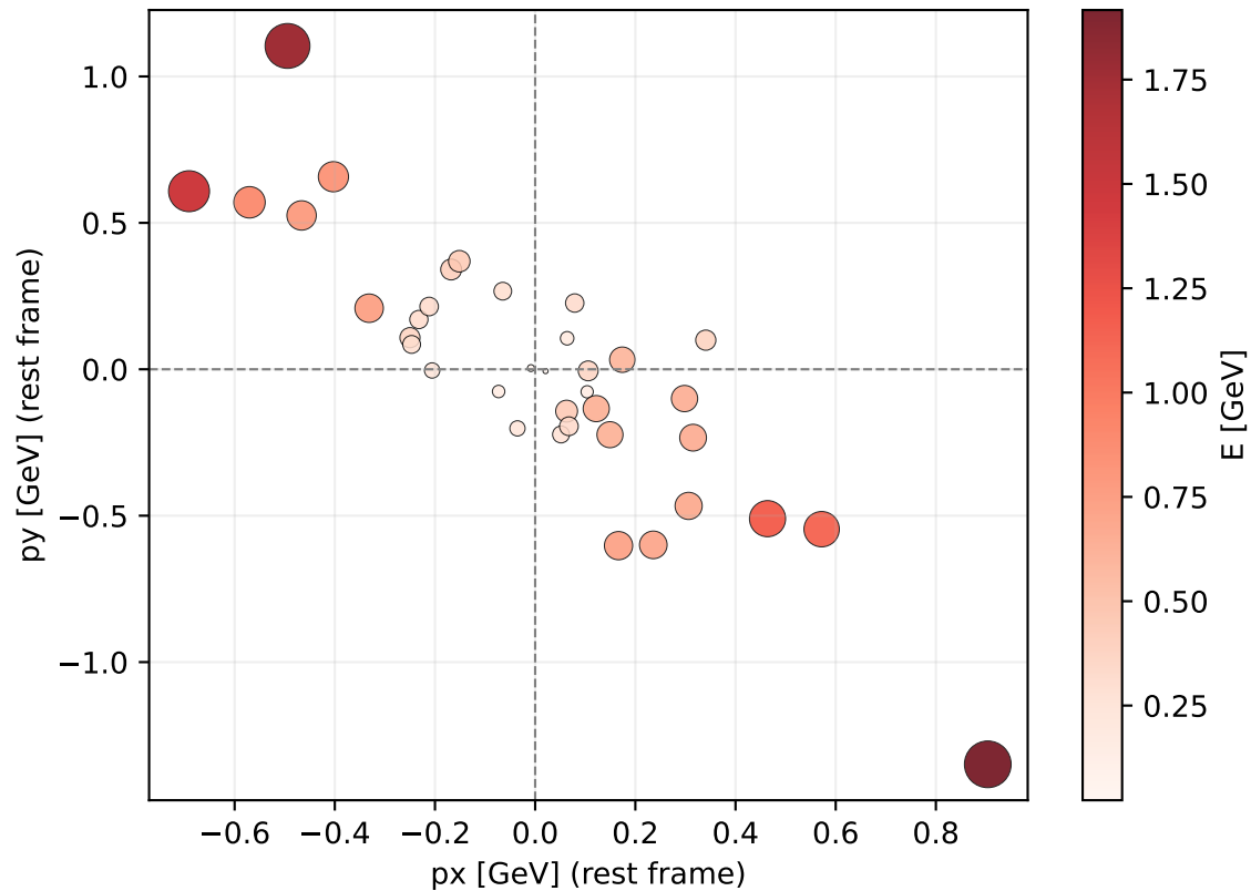
Gluon jet mult=37
