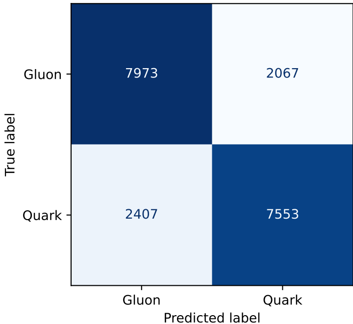
Confusion Matrix -- Rest-frame BDT (cut=0
