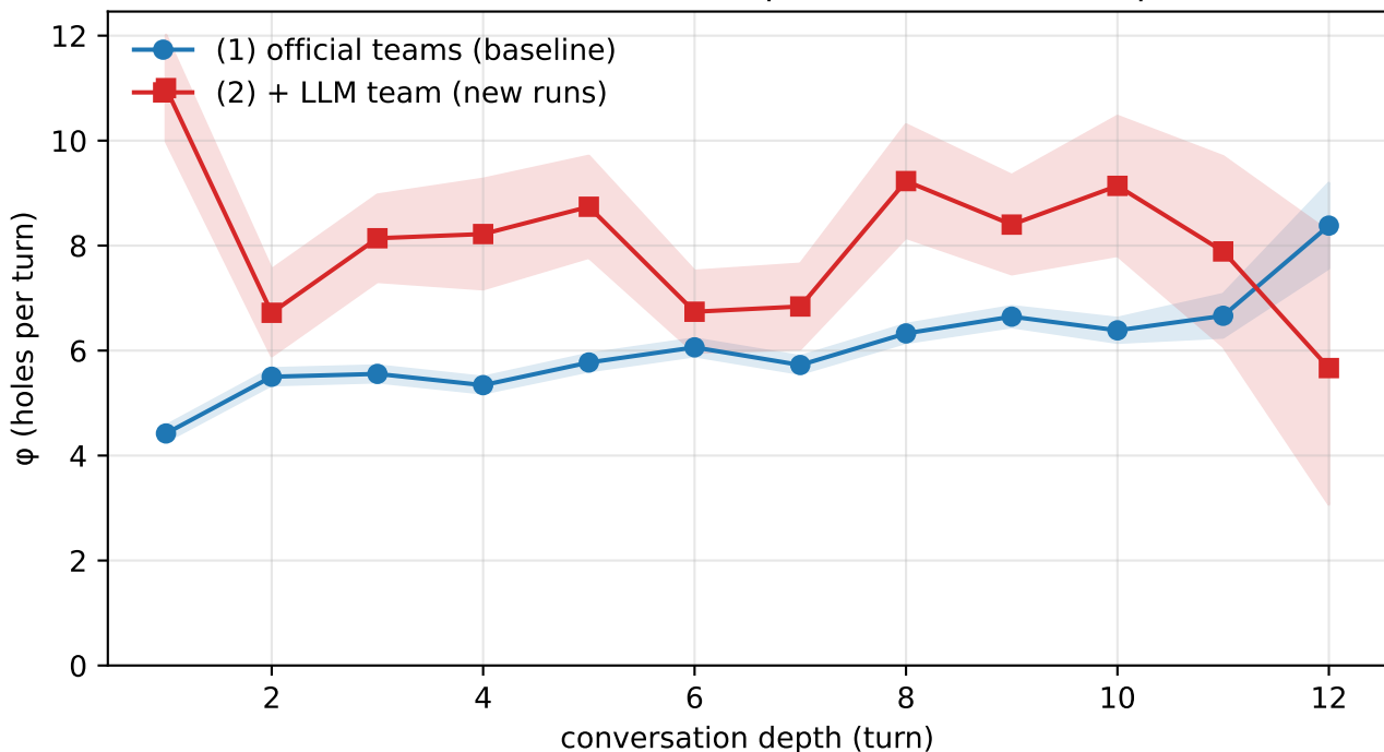
CAST2019: hole creation ( \phi ) vs conversation depth
