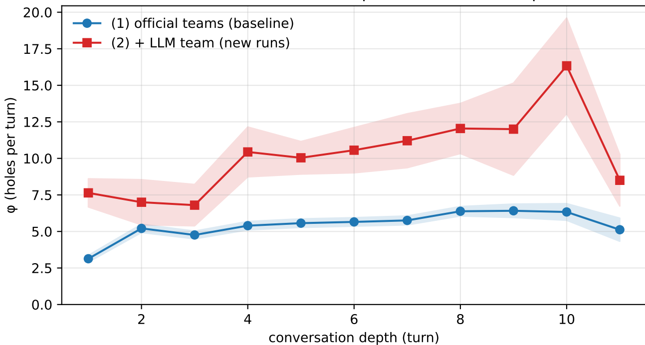
CAST2020: hole creation ( \phi ) vs conversation depth
