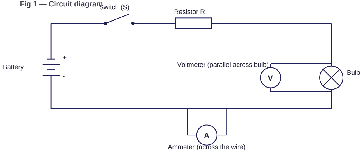
Fig 1 — Circuit diagram
