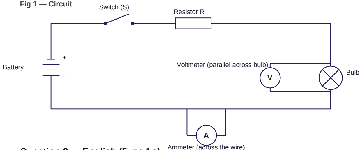
Fig 1 — Circuit
