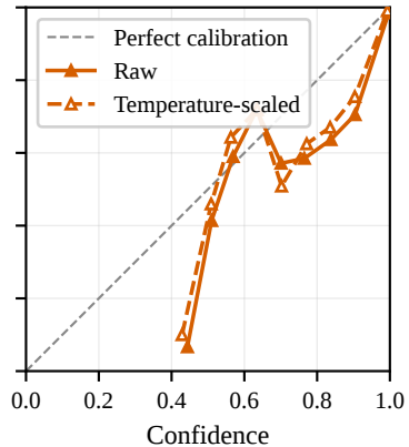
(c) ViT-B/16
