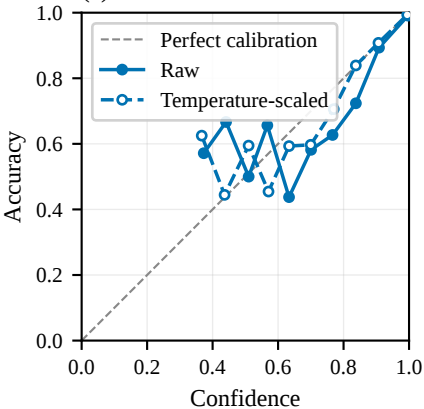
(a) ResNet18
