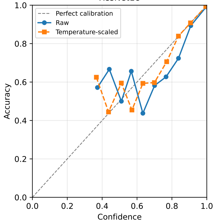
ResNet18
