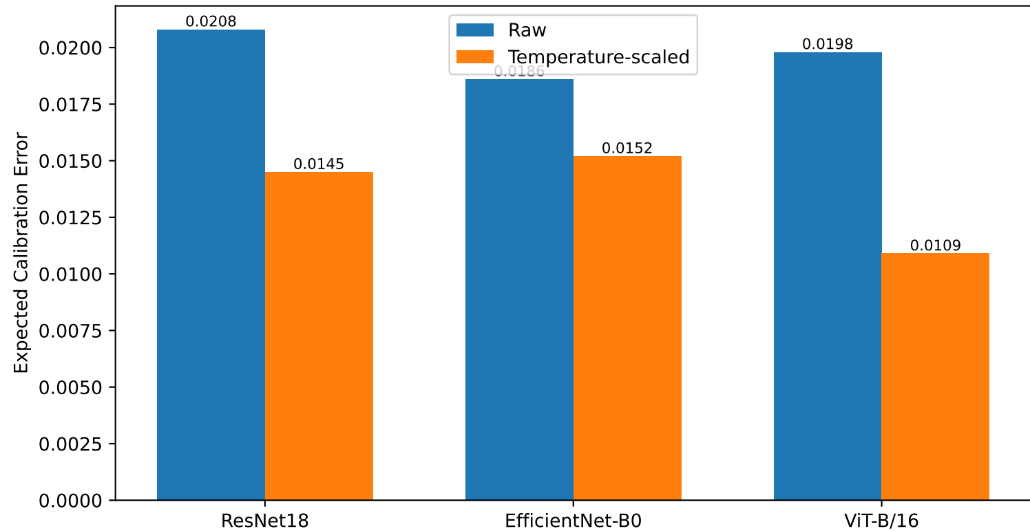
Internal D1 Calibration: ECE Before and After Temperature Scaling
