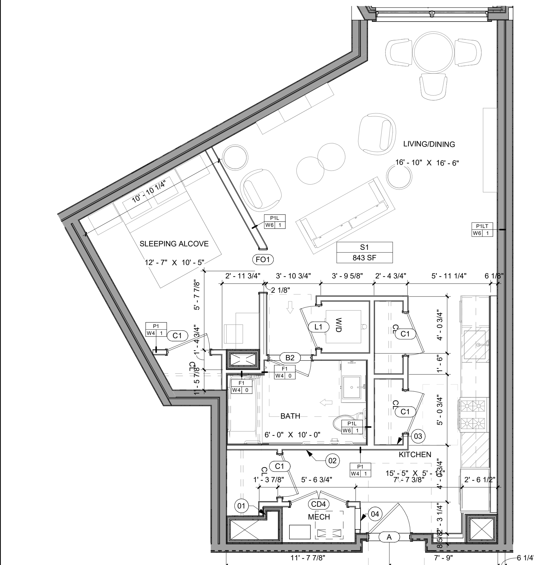
7 UNIT TYPE S1 SCALE: 1/4" = 1'-0"
