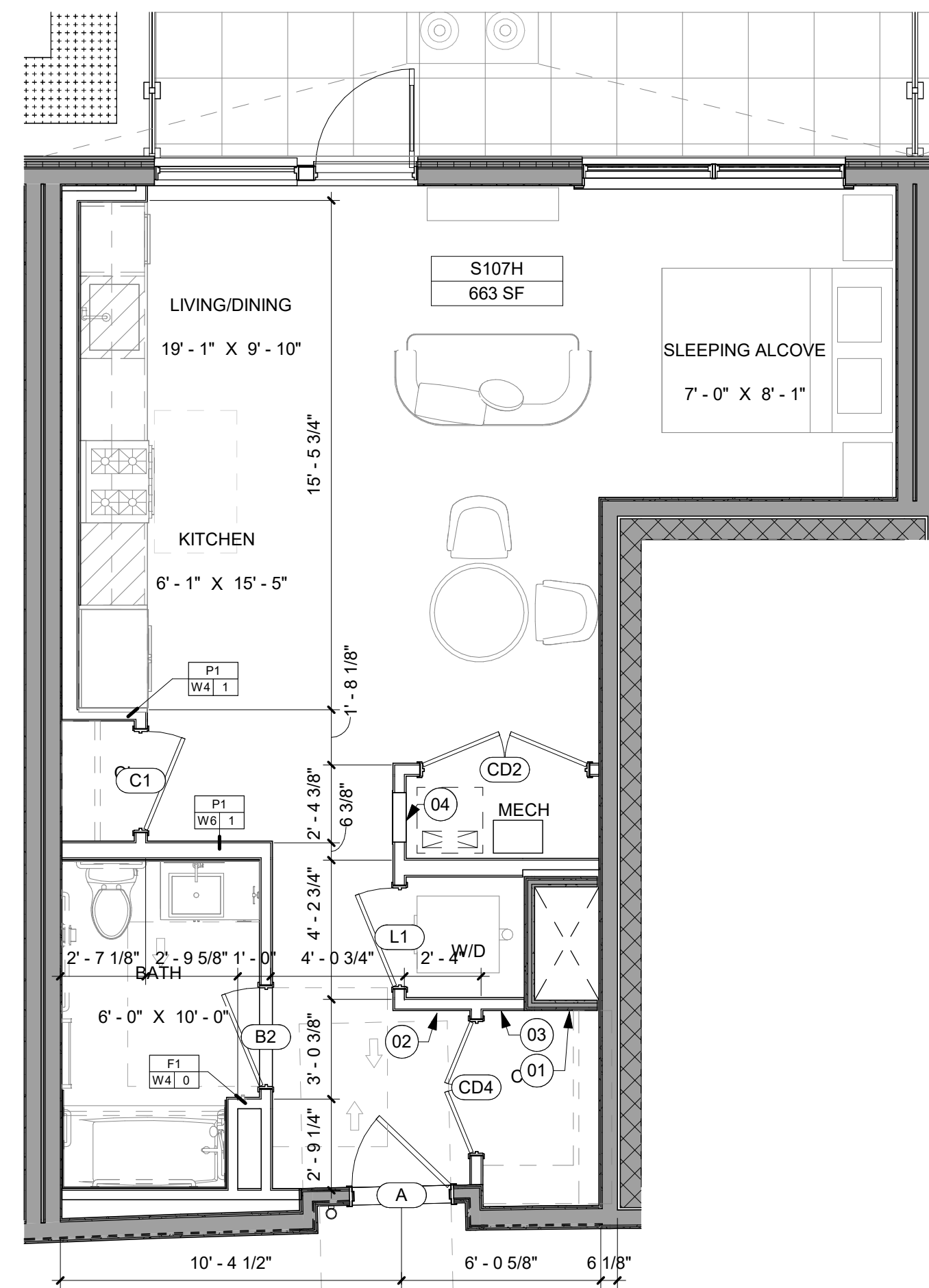
1 UNIT TYPE - S107H SCALE: 1/4" = 1'-0" UNIT TYPE KITCHEN TYPE BATHROOM TYPE COUNT AREA S107H K6 B1 3 663 SF
