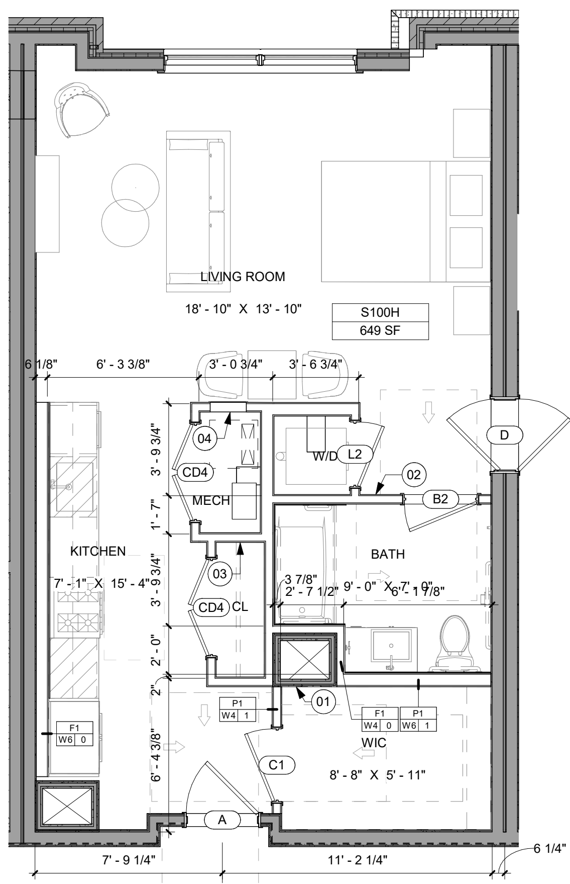
8 UNIT TYPE - S100H SCALE: 1/4" = 1'-0" UNIT TYPE KITCHEN TYPE BATHROOM TYPE COUNT AREA S100H K6 B1 8 649 SF ... 649 SF
