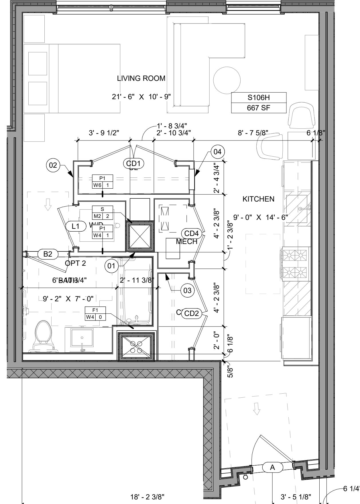
2 UNIT TYPE - S106H SCALE: 1/4" = 1'-0" UNIT TYPE KITCHEN TYPE BATHROOM TYPE COUNT AREA S106H K7 B3 3 667 SF
