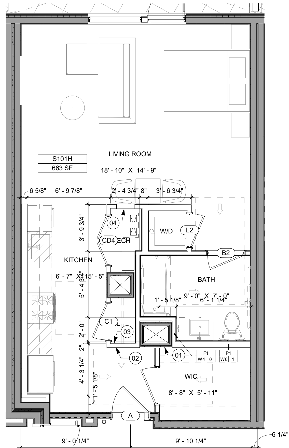
7 UNIT TYPE - S101H SCALE: 1/4" = 1'-0" UNIT TYPE KITCHEN TYPE BATHROOM TYPE COUNT AREA S101H K6 B1 3 656 SF ... 663 SF
