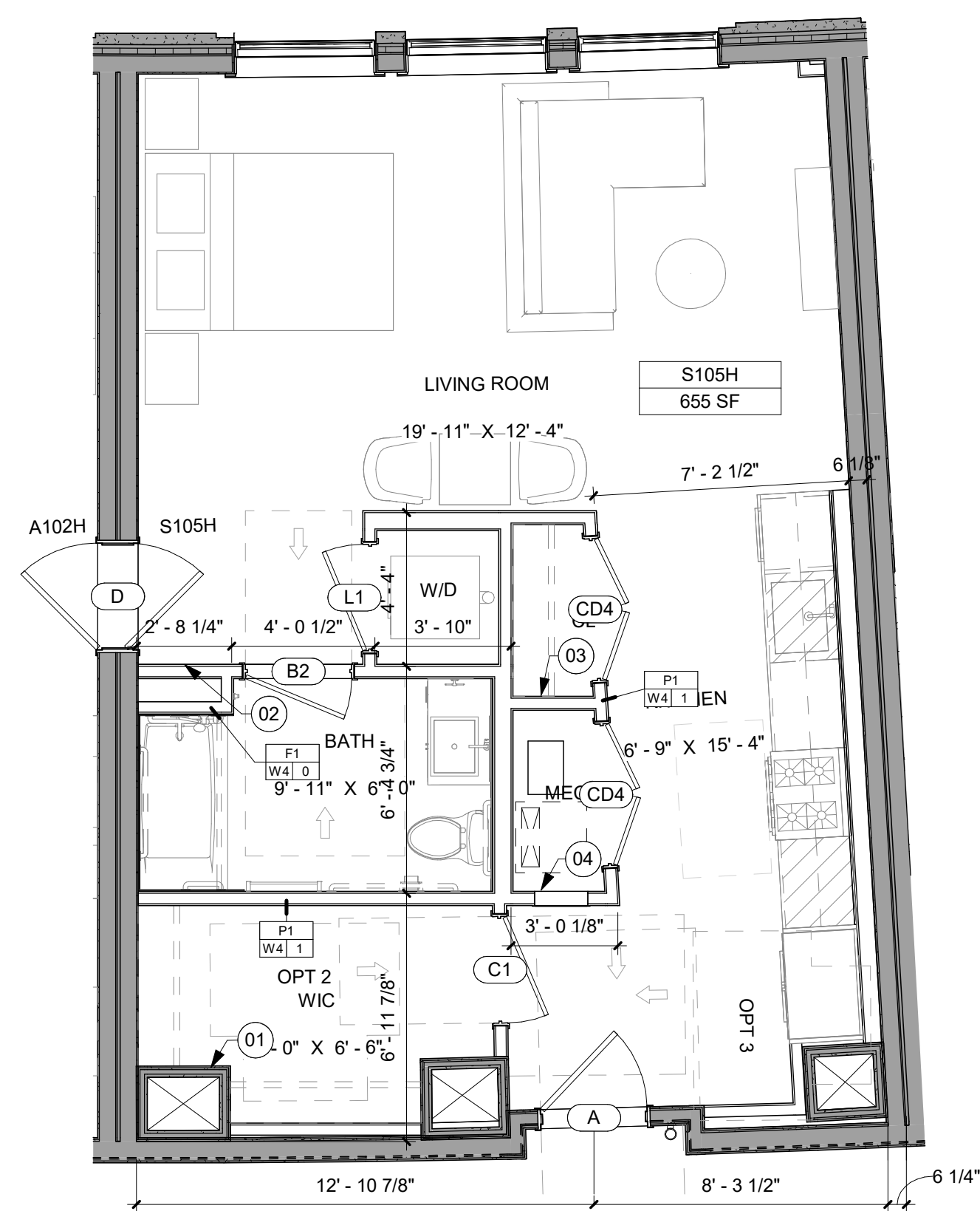
3 UNIT TYPE - S105H SCALE: 1/4" = 1'-0" UNIT TYPE KITCHEN TYPE BATHROOM TYPE COUNT AREA S105H K6 B2 3 655 SF ... 656 SF
