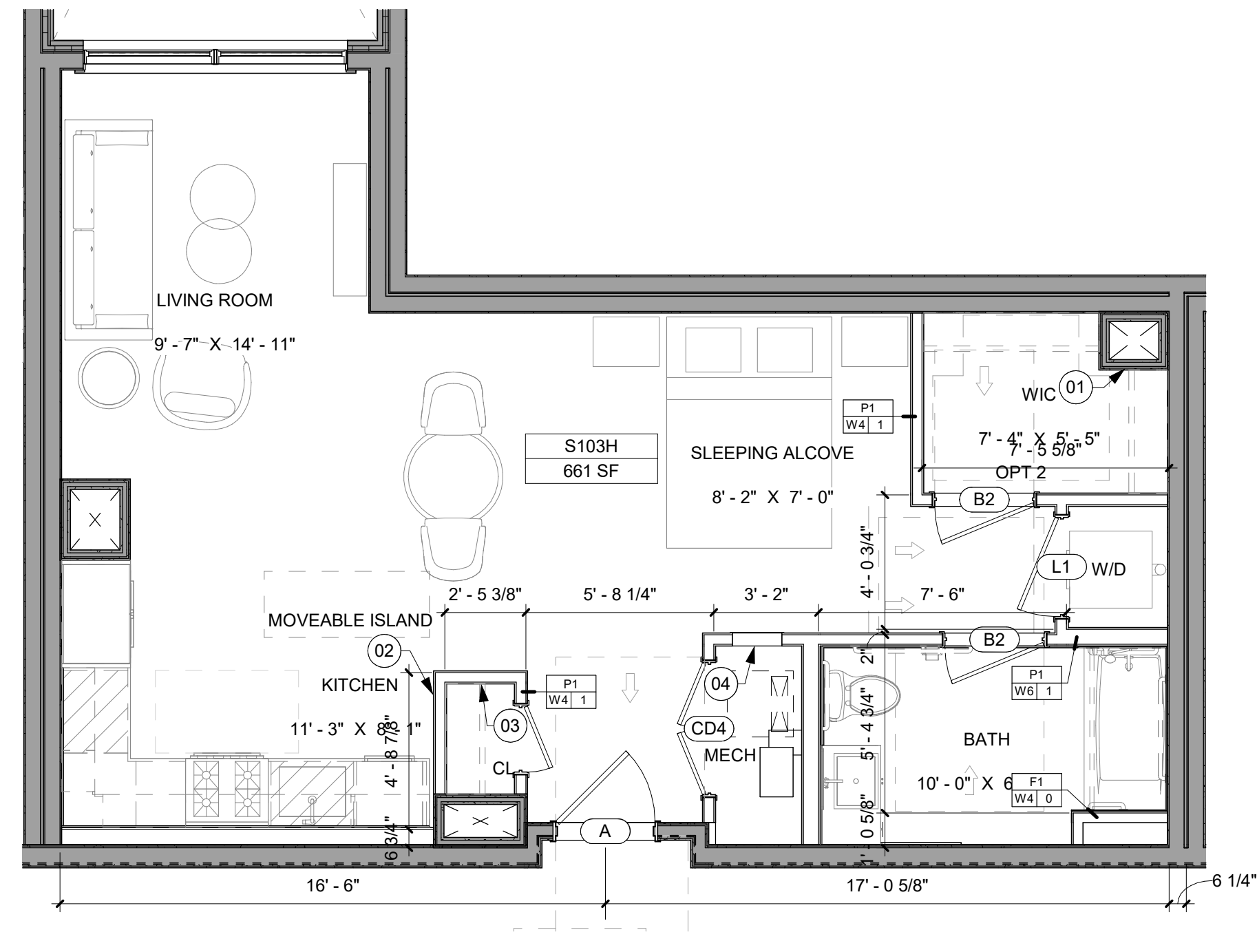
5 UNIT TYPE - S103H SCALE: 1/4" = 1'-0" UNIT TYPE KITCHEN TYPE BATHROOM TYPE COUNT AREA S103H K6 K1 4 661 SF ... 665 SF
