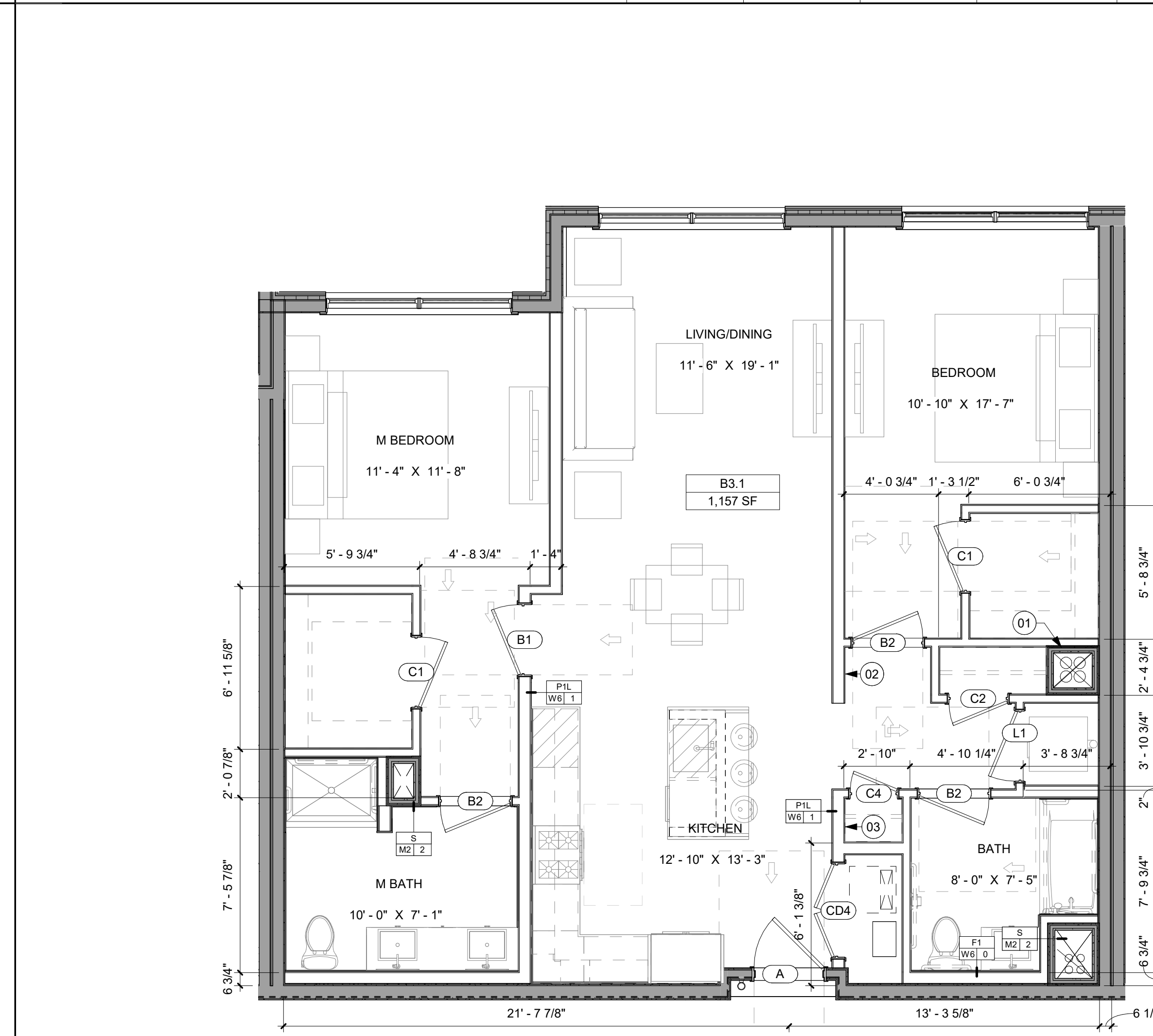
5 UPF - UNIT TYPE B3.1 SCALE: 1/4" = 1'-0"
