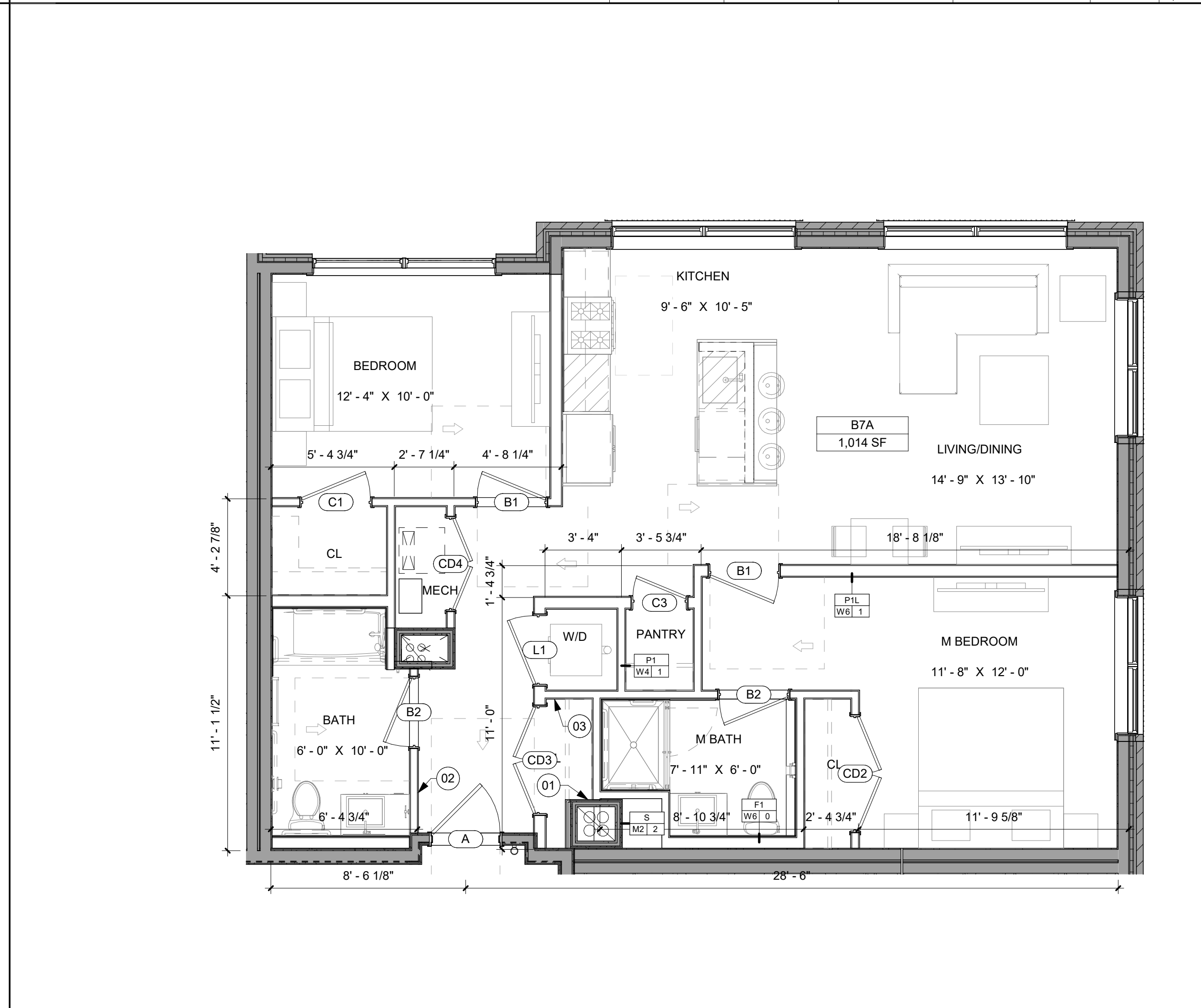
1 UNIT TYPE - B7A - AFF SCALE: 1/4" = 1'-0"
