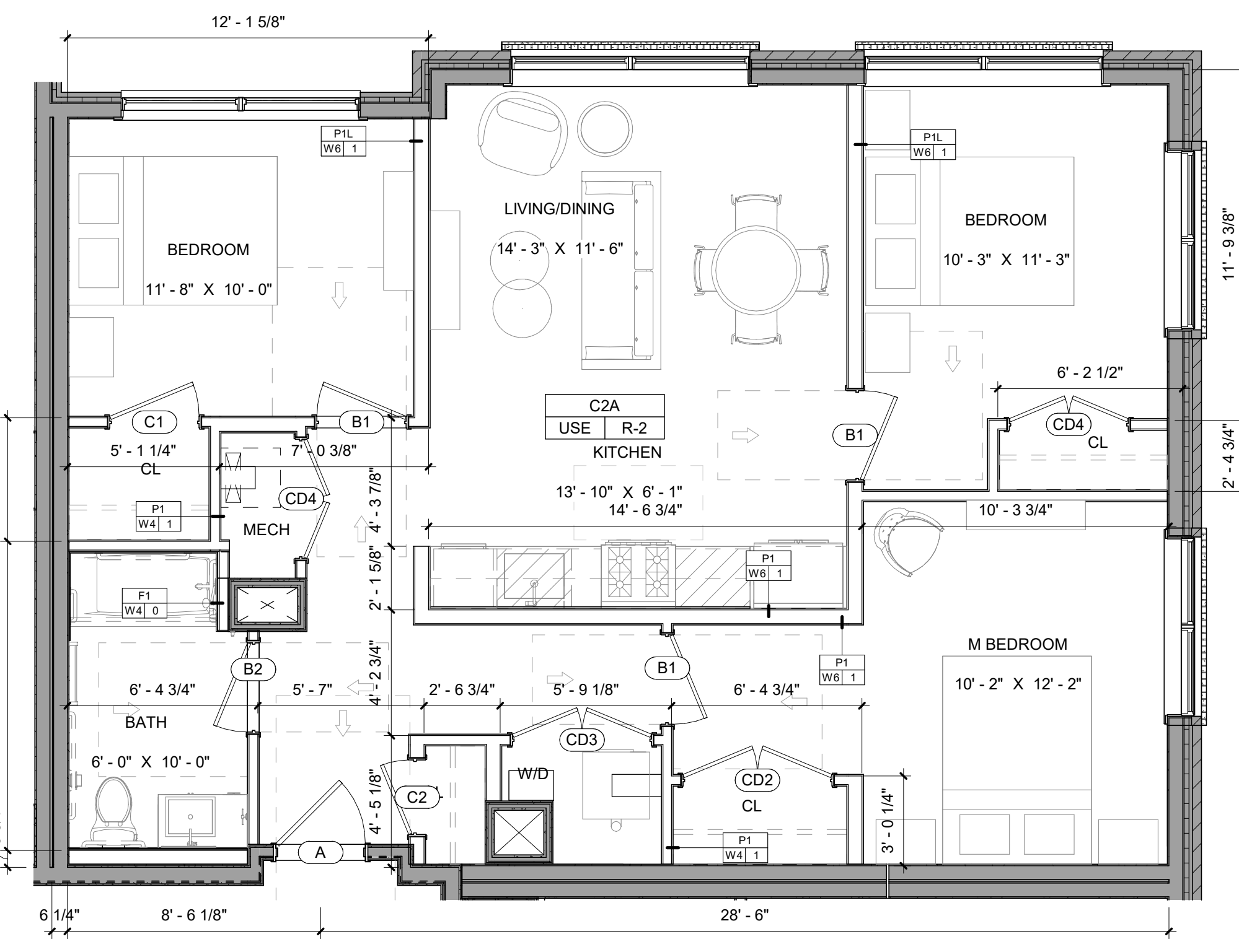
1 UNIT TYPE - C2A - AFF SCALE: 1/4" = 1'-0"
