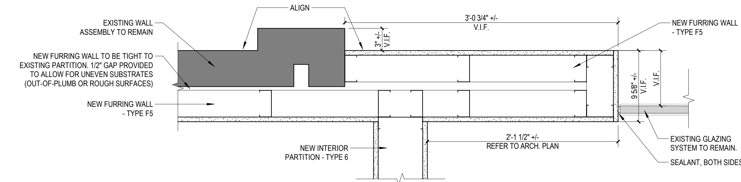
2D PLAN DETAIL - MODIFIED EXISTING GLAZING SYSTEM 1 1/2" = 1'-0"
