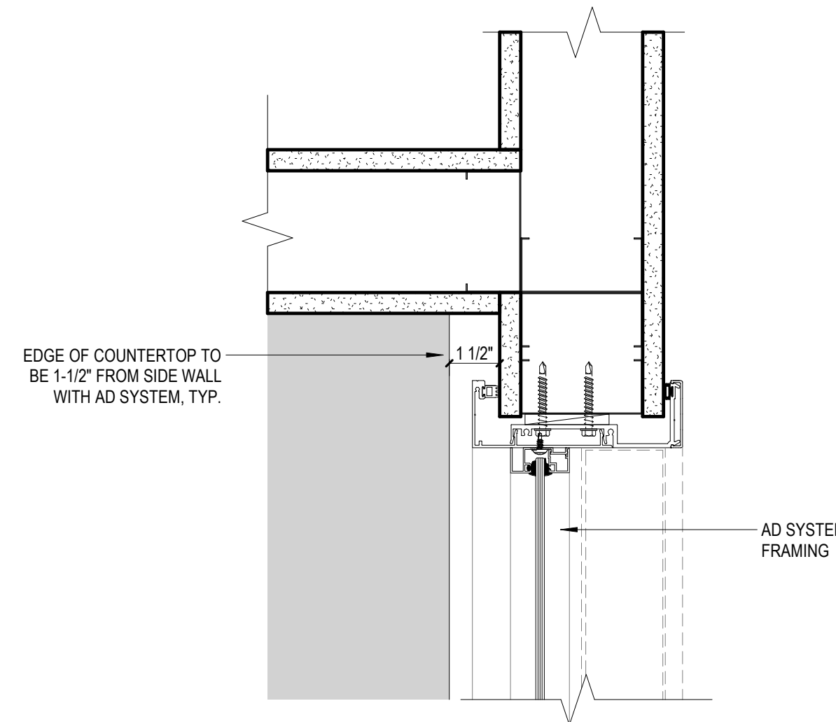
4D PLAN DETAIL - CORNER AT PHYSICIAN TOUCHDOWN, TYP. 3" = 1'-0"
