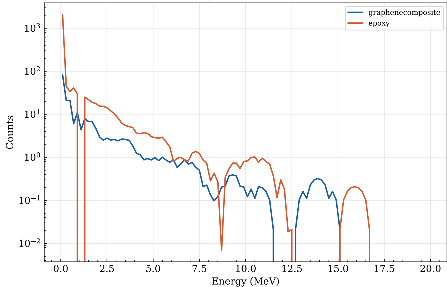
Shielding Material Comparison
