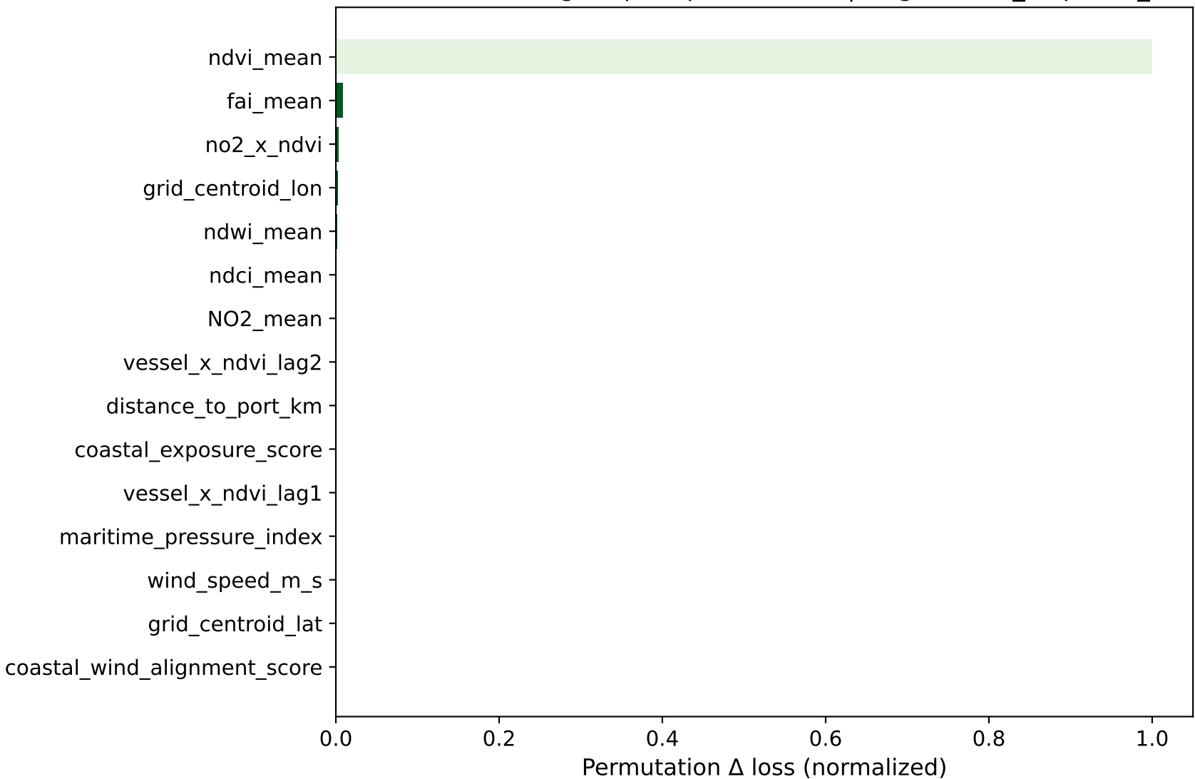
HistGradientBoosting · top 15 permutation | target=land_response_index
