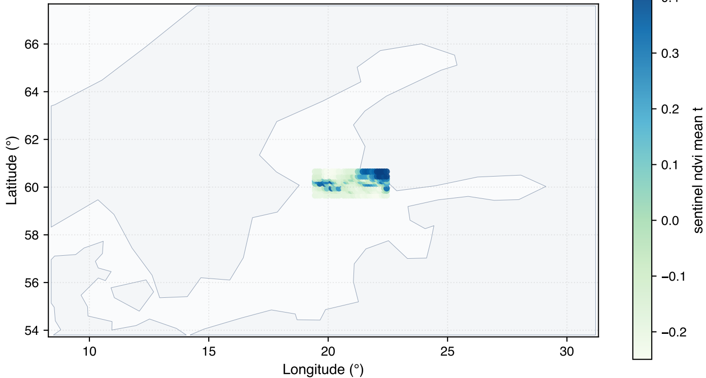
NDVI mean (week t)
