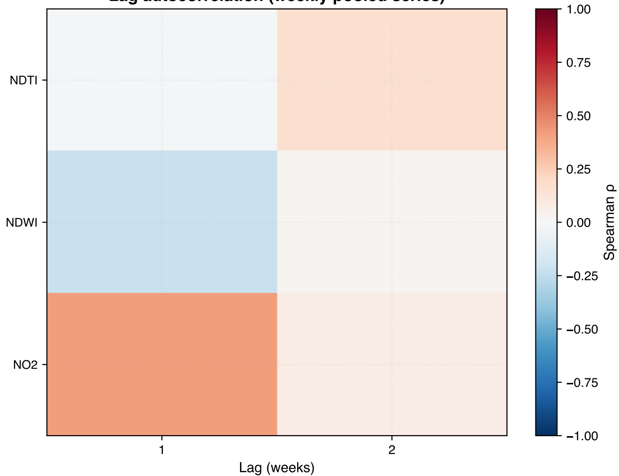
Lag autocorrelation (weekly pooled series)
