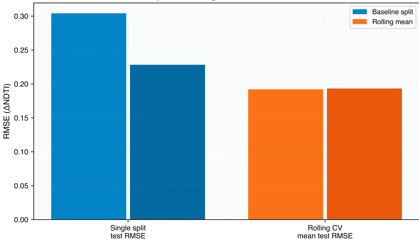
Standard split vs rolling-window CV — \Delta NDTI RMSE
