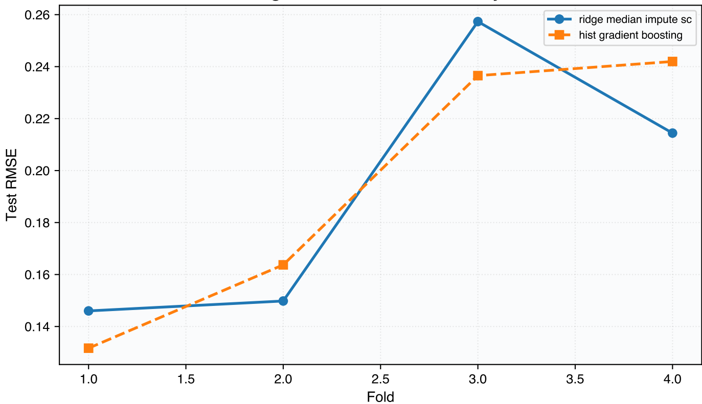
Rolling CV — \Delta NDTI test RMSE by fold
