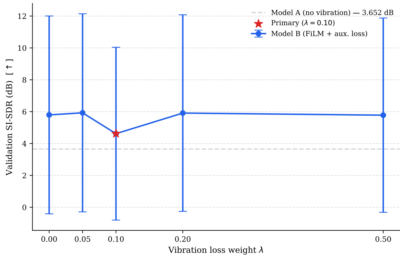
Ablation: Effect of Vibration Loss Weight \lambda
