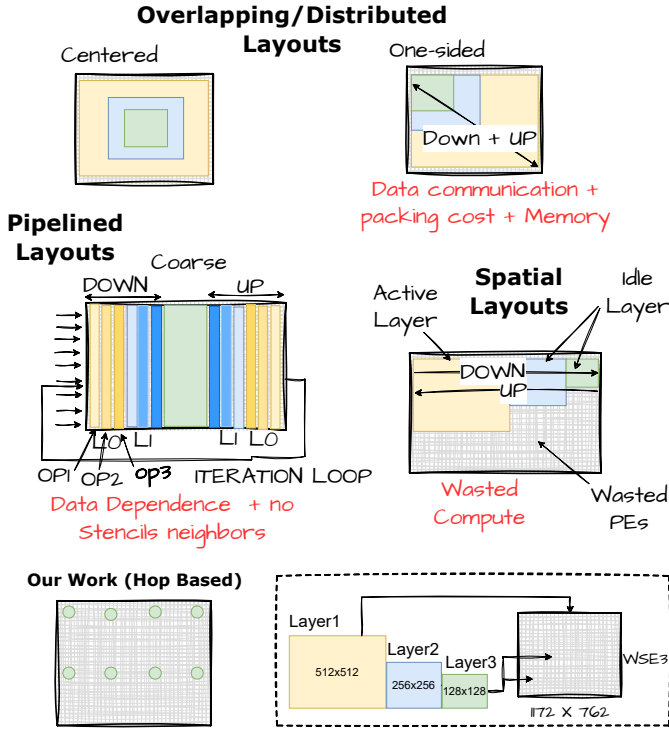
Fig. 3. Different possible layouts for 3 level GMG layers on WSE3 of size 1172x762. Text in red highlights various challenges of each approach. Our approach falls into the distributed category.
