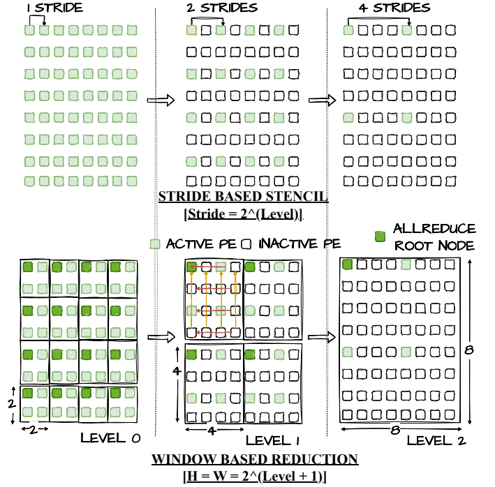
Fig. 4. Top: Stencil Operator on WSE-3 2D grid for a 8^3 problem with 3 levels. The Highlighted nodes are the Active PEs and remaining Inactive PEs. The Hop distance differs as one keeps going down the levels and the SpMV exchanges halo regions H hops apart
