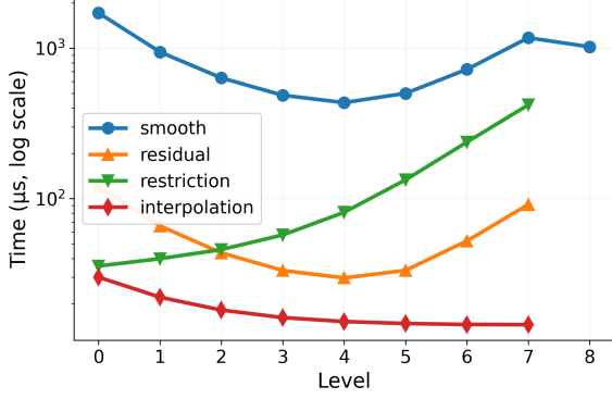
Fig. 6. Per-operator time per level for one V-cycle on a 512^3 problem (GLOW on CS-3). Down and up phases are summed at each level. x -axis: level 0 (finest) to 8 (coarsest). y -axis: time (log scale; higher is slower). Config: 4/4/6 pre/post/coarse, 9 levels, FP32, 7-point stencil.
