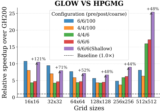
Fig. 5. Speedup comparison between Cerebras CS-3 and NVIDIA GH200 using HPGMG/Glow across various problem sizes. The bar plot shows relative performance (higher is better). The % increase indicated on top of 6/6/6(Shallow)(purple) is the relative speedup against the 6/6/6(red),
