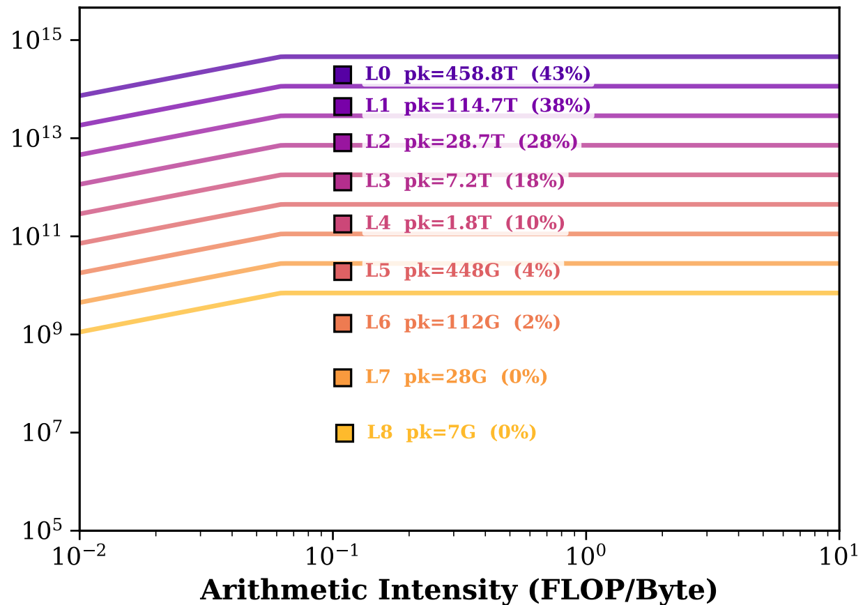
(b) Active-PE System (per-level peak)
