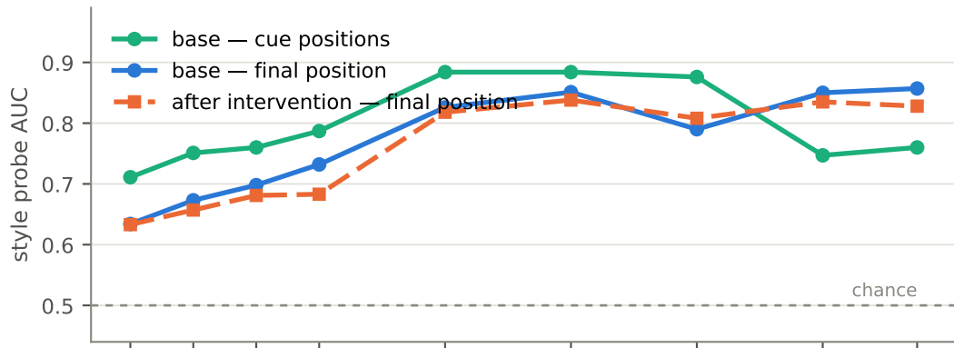
b No layer survives the cluster permutation test ( n = 15 units); bound 0.107 AUC
