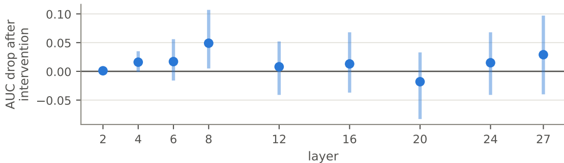
b No layer survives the cluster permutation test ( n = 15 units); bound 0.107 AUC
