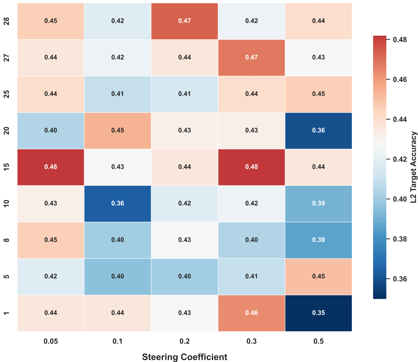
Raw Steering: L2 Target Accuracy (baseline = 0.43, n=220)
