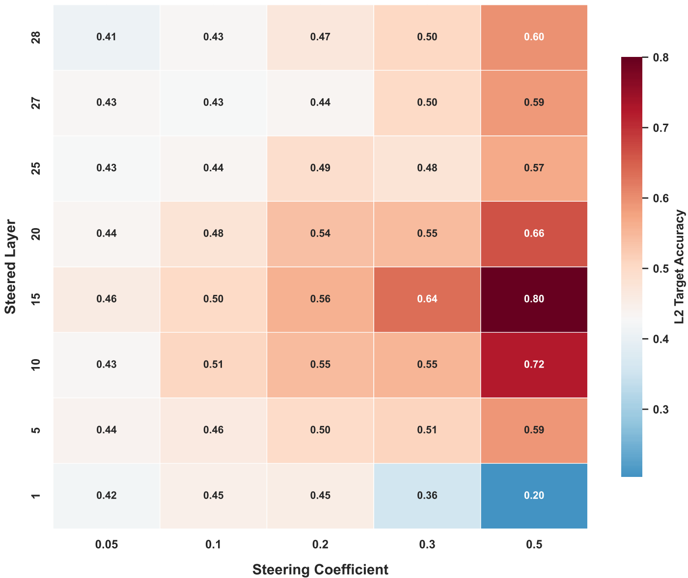
Contrastive Steering: L2 Target Accuracy (baseline = 0.43, n=220)
