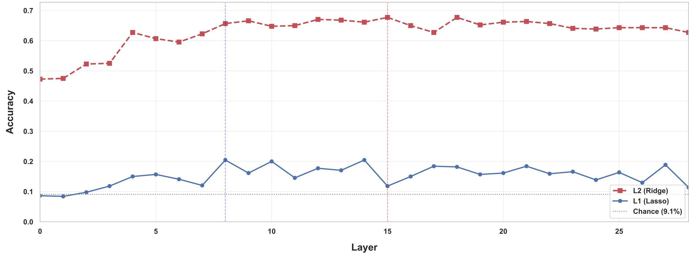
Probing Accuracy Per Layer — Prompt Embeddings (Llama-3.2-3B-Instruct)
