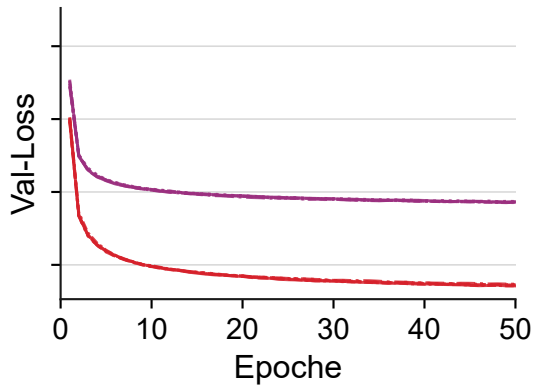
Val-Loss
