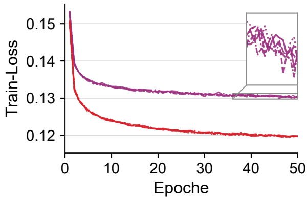
Train-Loss
