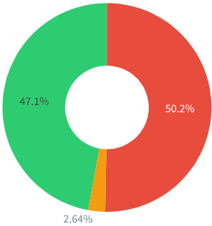
Sentiment Distribution
