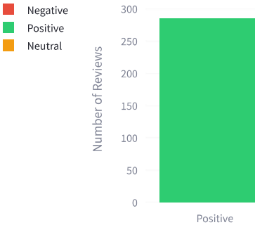
Review Counts
