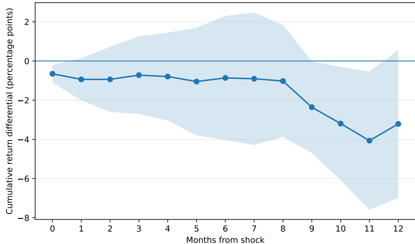
External financing dependence: Continuous CPU \times VIX activation
