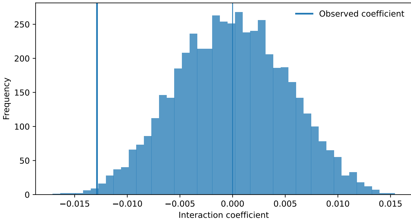
Permutation distribution: Growth Duration Exposure Final Cpu And Vix Stress
