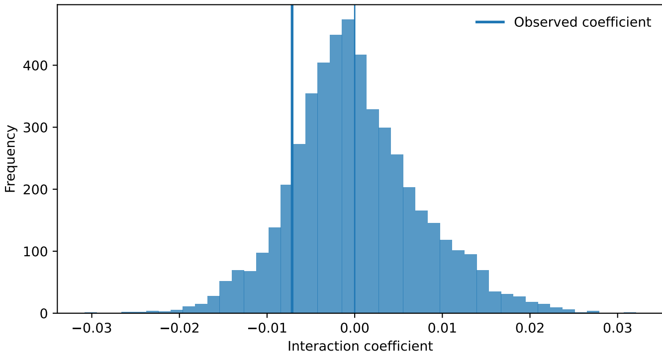
Permutation distribution: Internal Financial Capacity Cpu And Vix Stress
