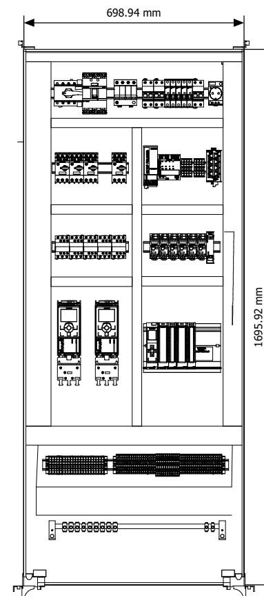
FRONT MONTING PANEL VIEW
