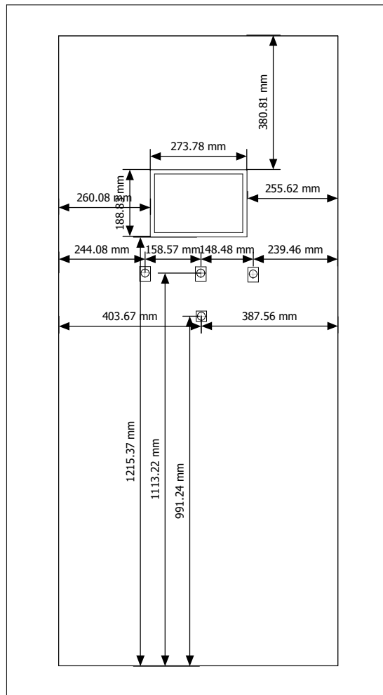
DOOR DRILLING VIEW
