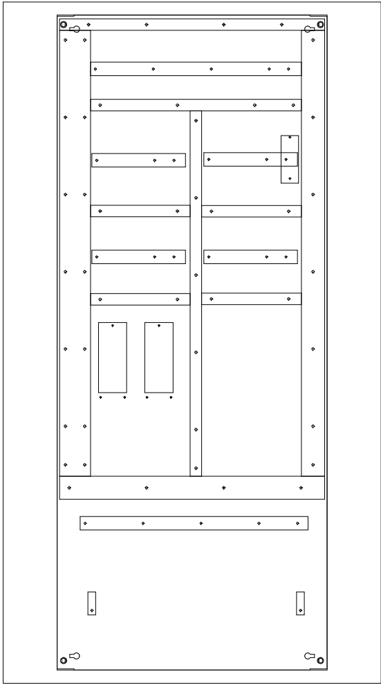
FRONT MONTING PANEL DRILLING VIEW
