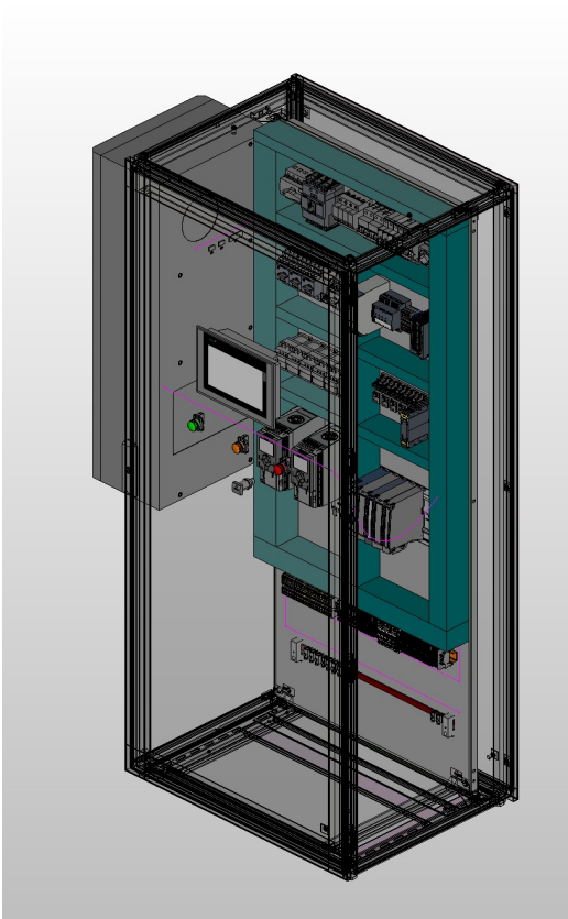
ENCLOUSURE VIEW
