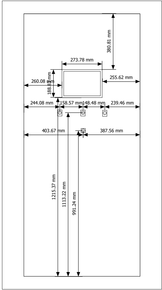
DOOR DRILLING VIEW
