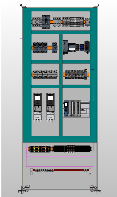
FRONT MONTING PANEL VIEW
