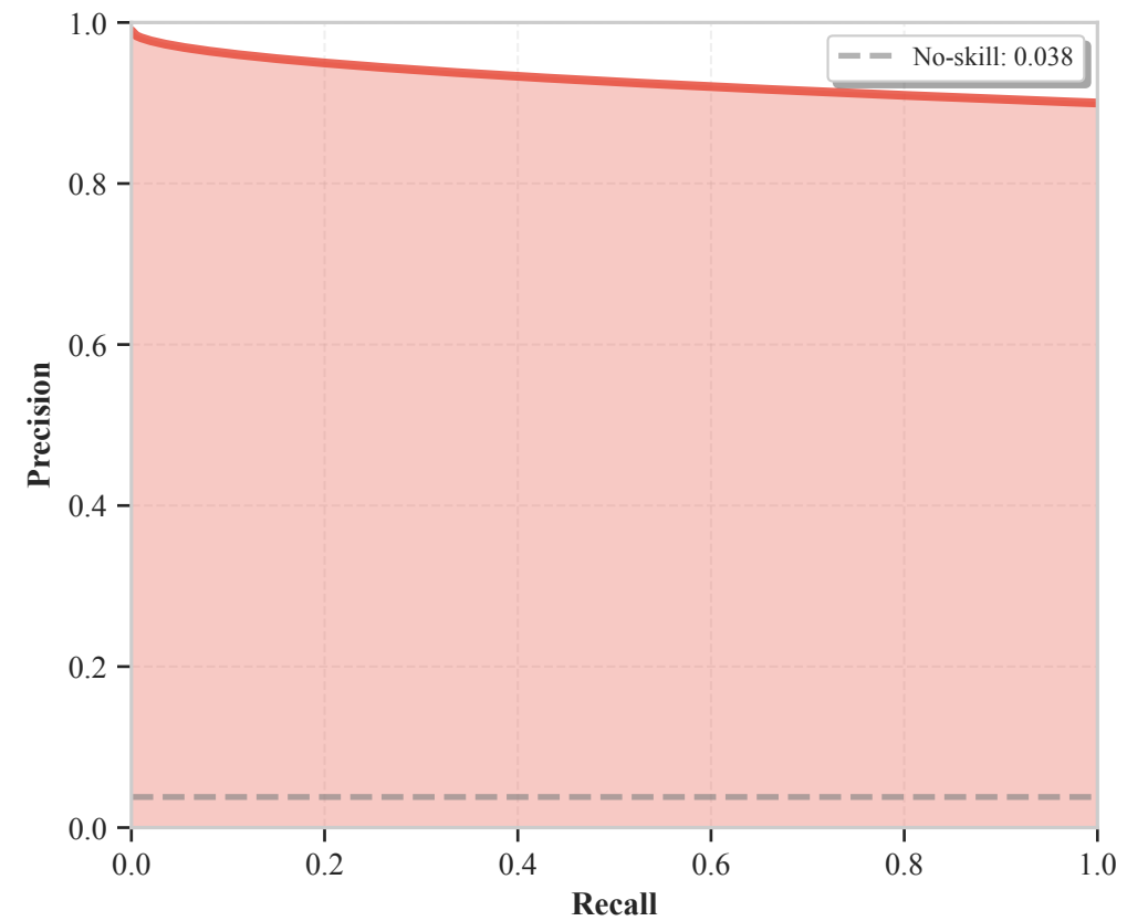
(c) Avoidant AP = 0.94
