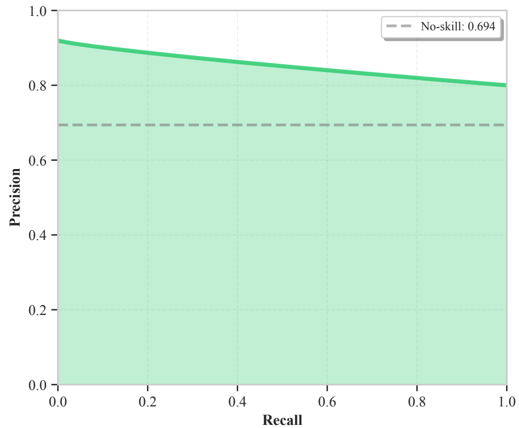
(a) Affiliative AP = 0.81
