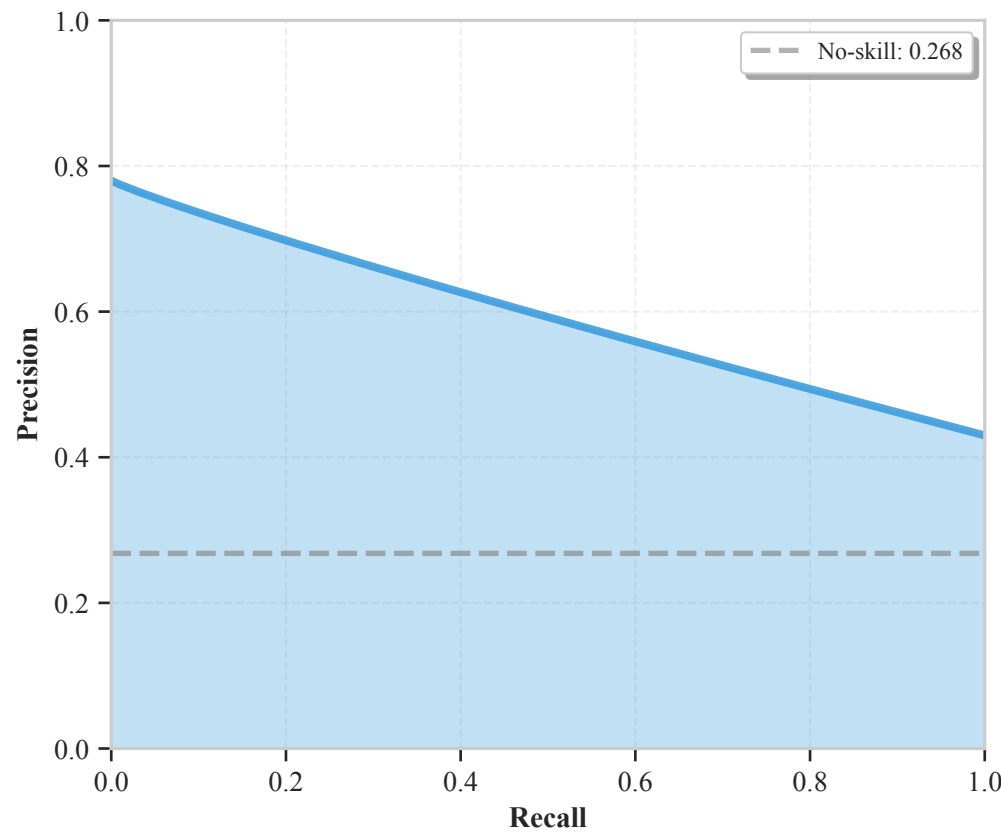
(b) Neutral AP = 0.65
