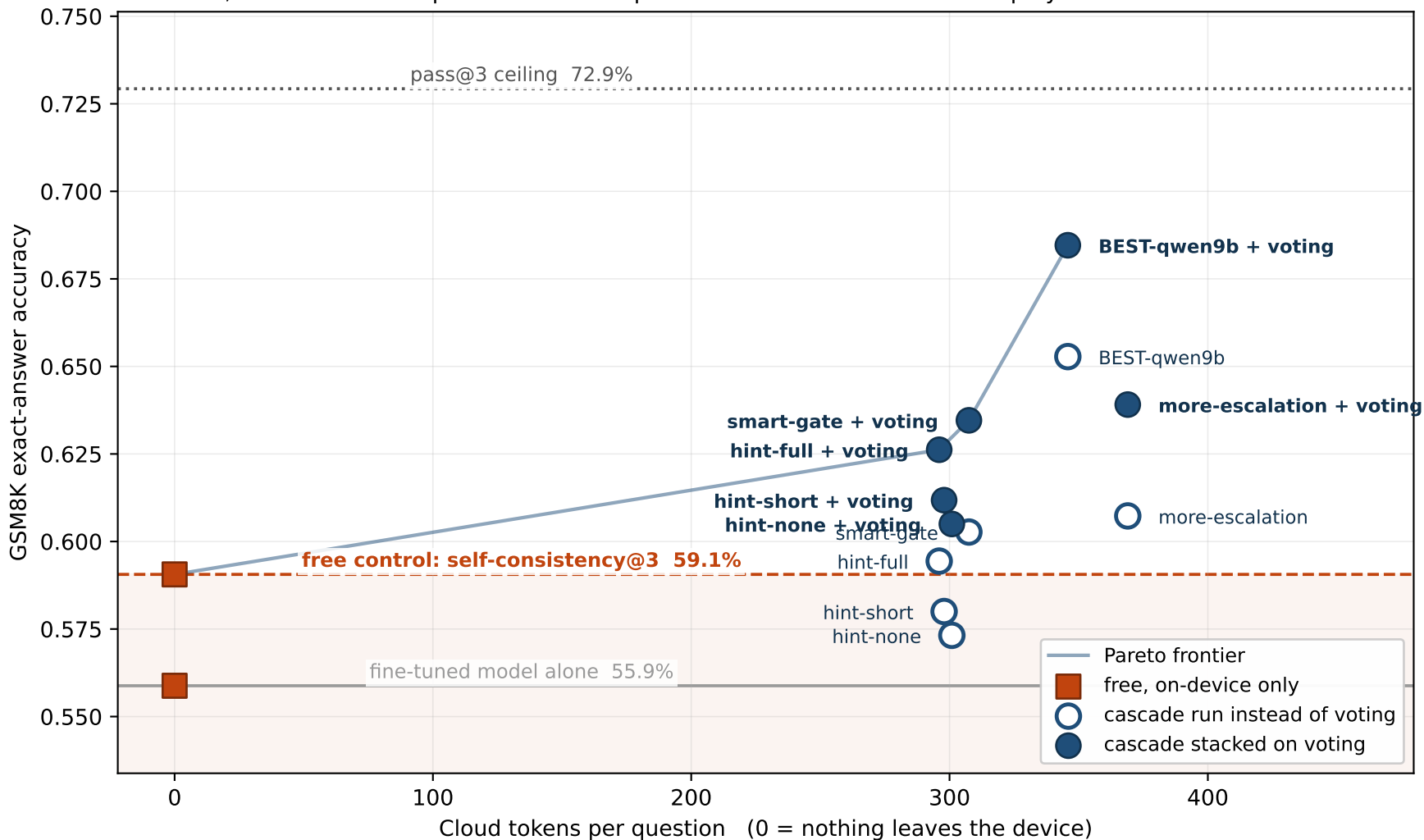
Accuracy vs. cloud cost: gemma-4-E2B-it with a GLM-4.7-Flash supervisor 1,319 GSM8K test questions. Hollow points are off the frontier - no deployer would choose them.
