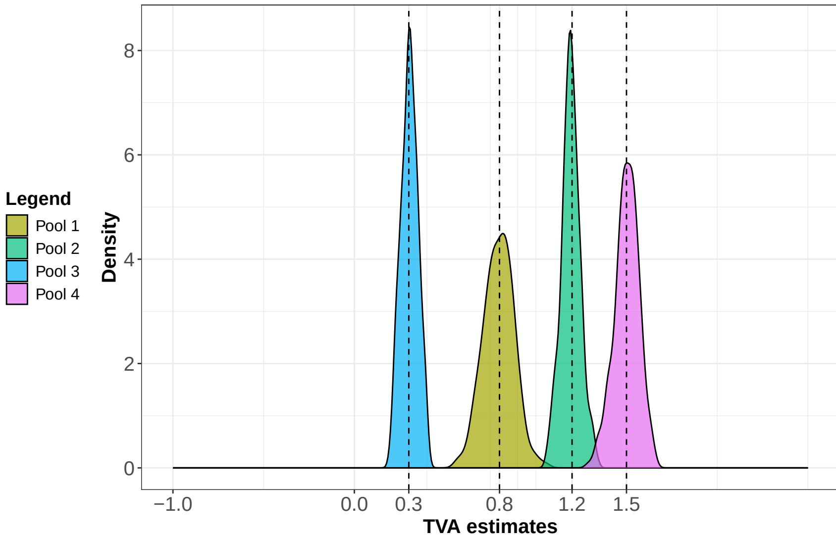
Distribution of TVA estimates by policy for 300 simulations
