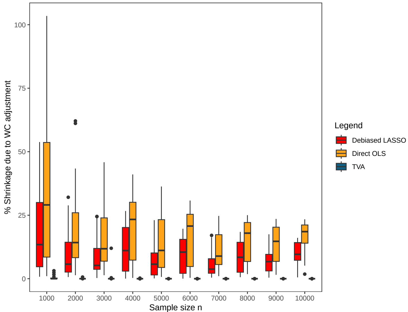
A Shrinkage imposed by WC adjustment
