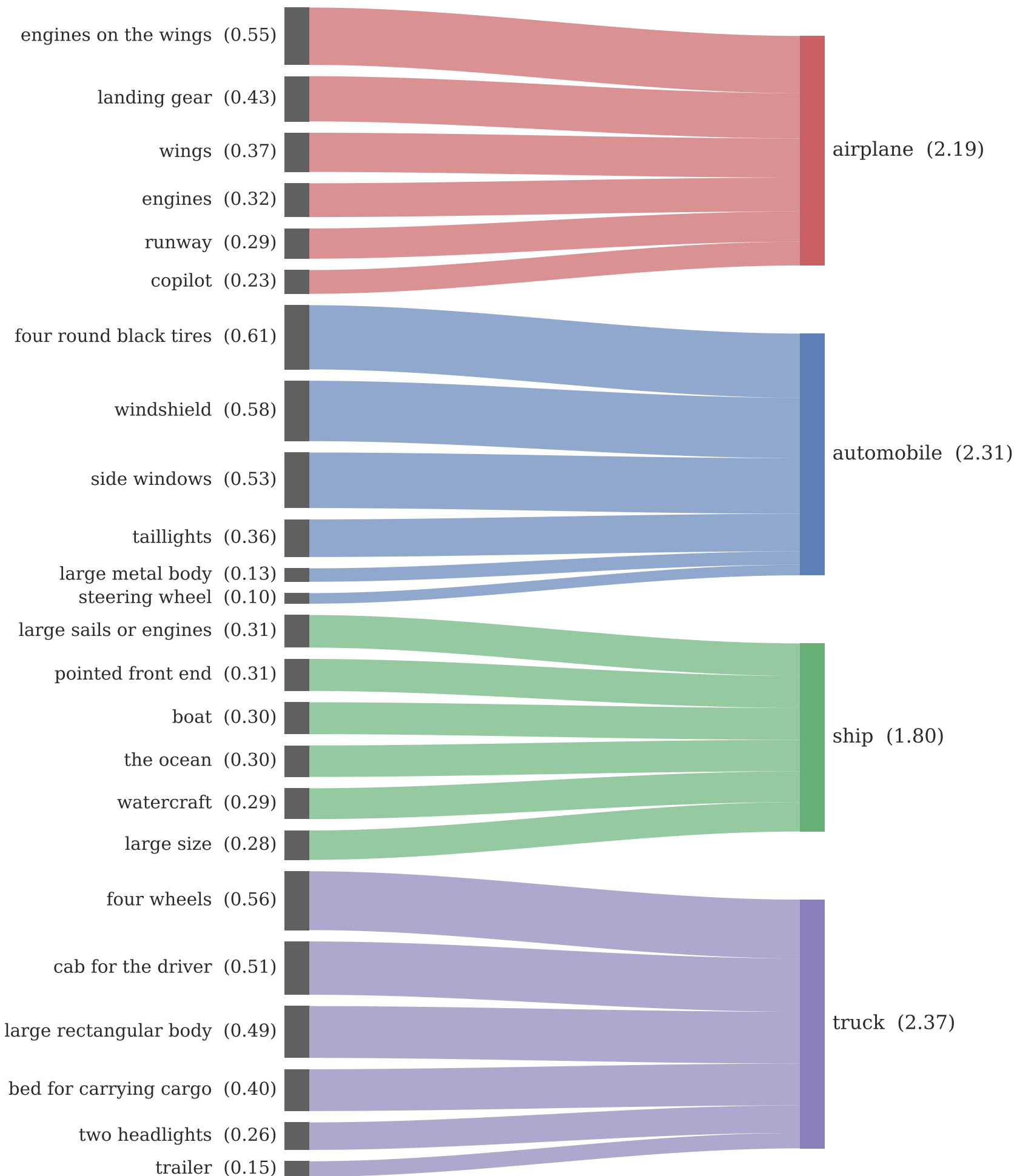
Concept-to-class weights: cifar10_vehicles
