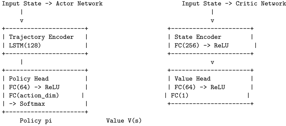
Figure 1: Architecture of A2C with Separate Networks
