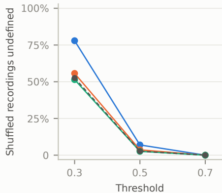
(c) Finch, undefined shuffled R^2
