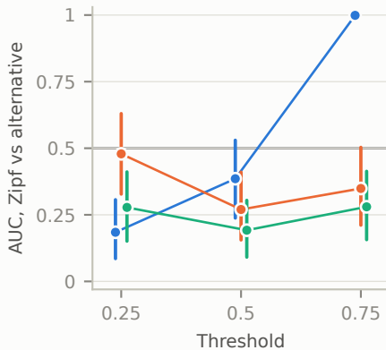
(b) Whale song, rotated z
