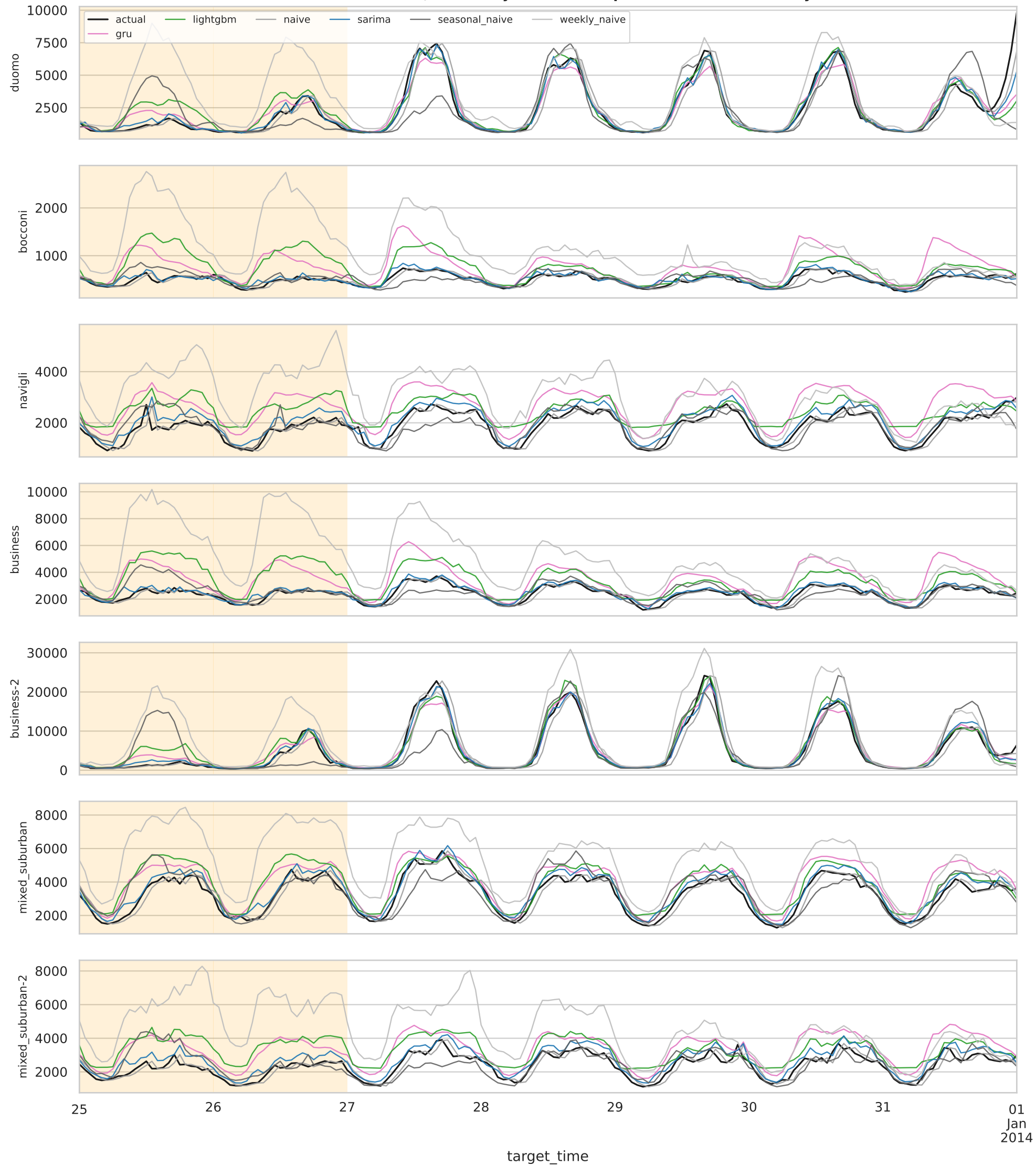
1 h-ahead forecasts, last 7 days of the test period (shaded = holidays)
