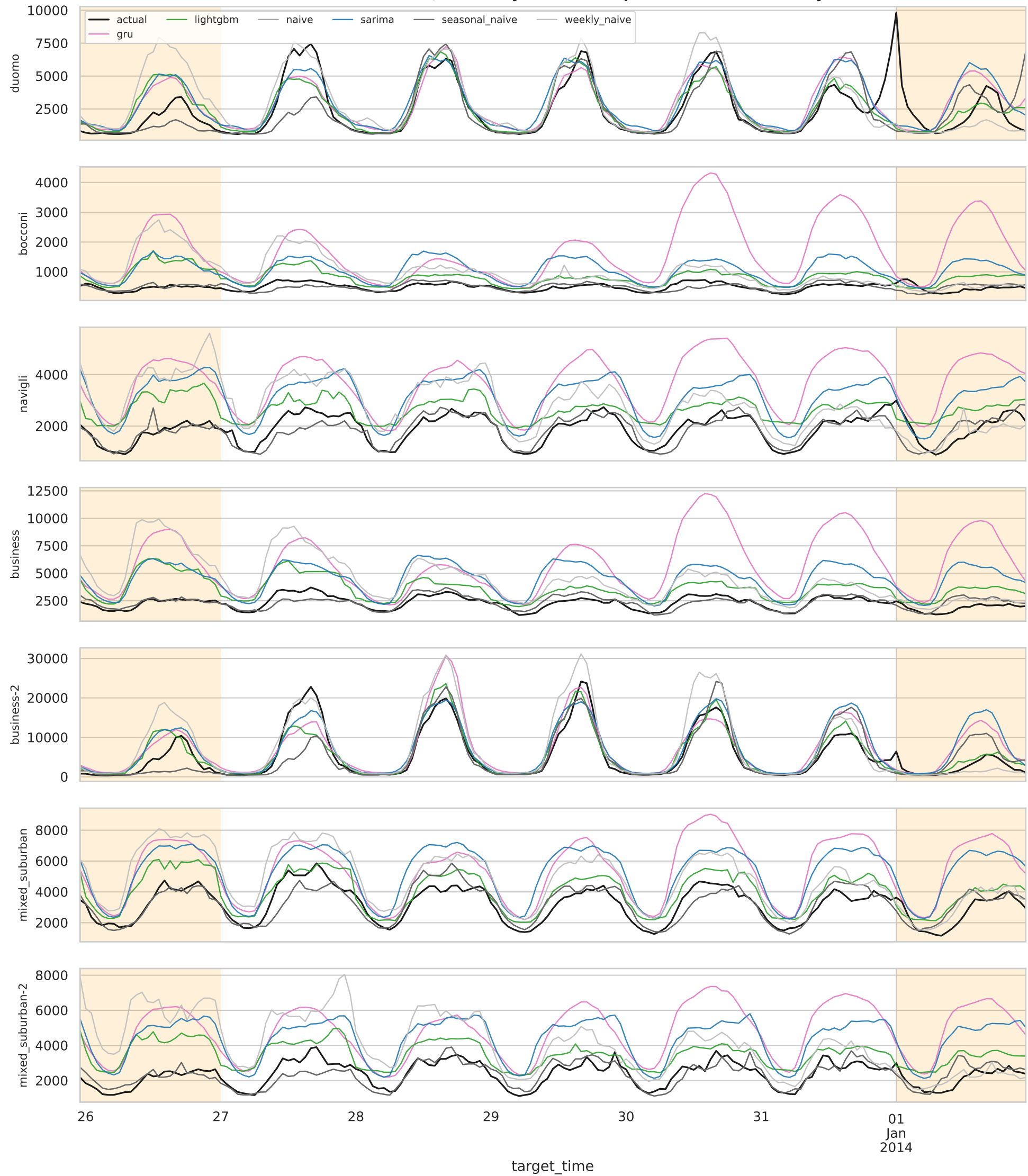
24 h-ahead forecasts, last 7 days of the test period (shaded = holidays)
