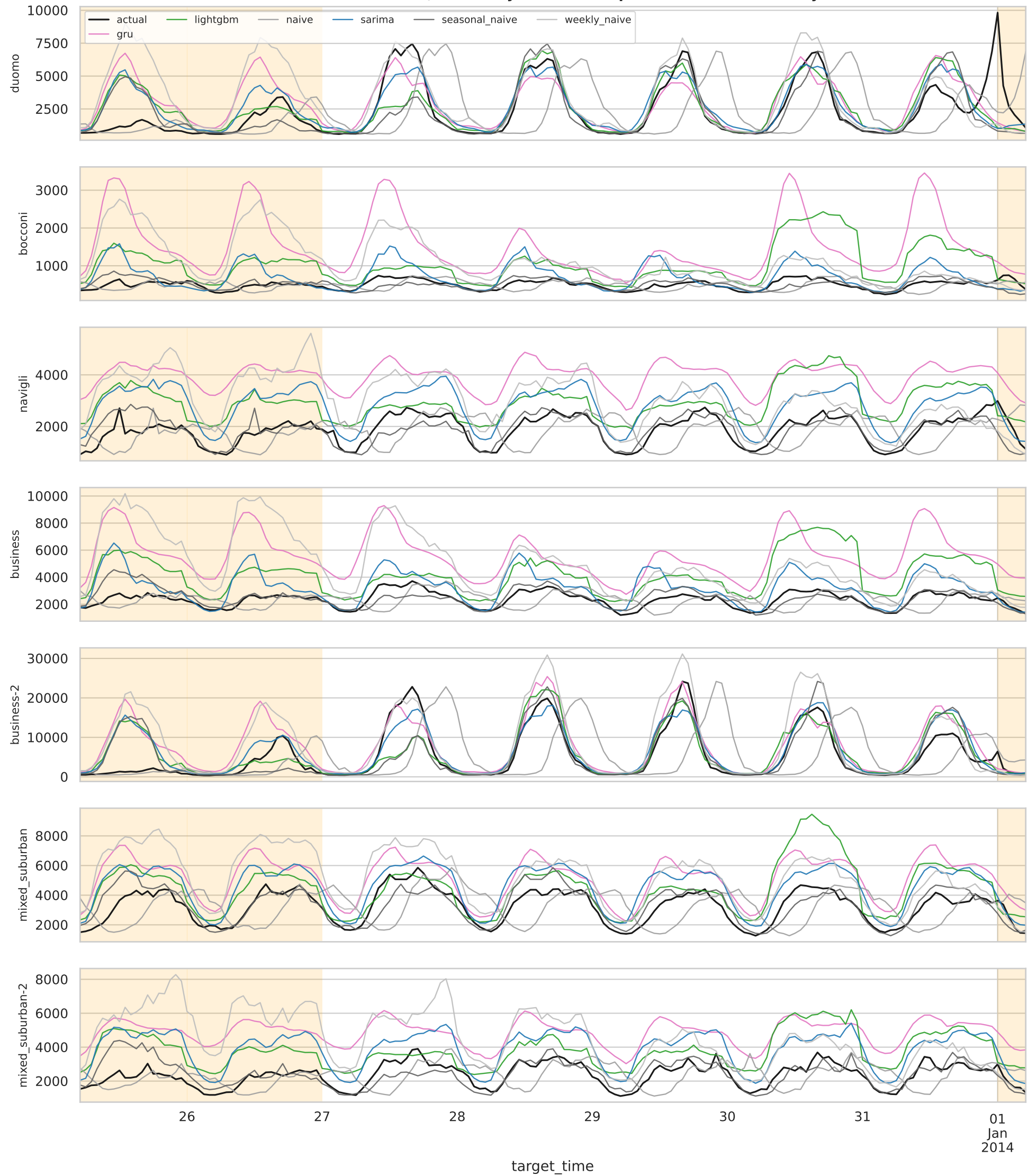
6 h-ahead forecasts, last 7 days of the test period (shaded = holidays)
