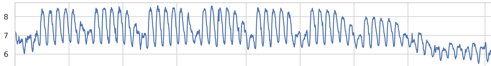
MSTL decomposition (24 h and 168 h) of \log(1+\text{bocconi})
