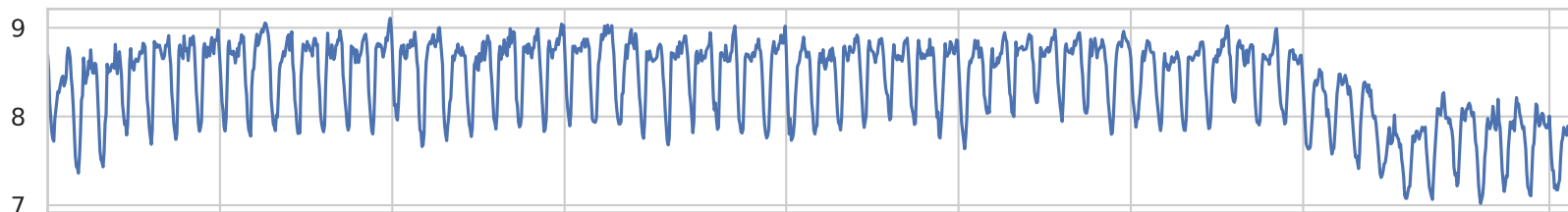
MSTL decomposition (24 h and 168 h) of \log(1+\text{mixed\_suburban-2})
