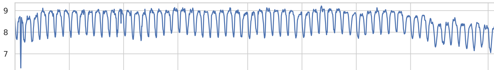
MSTL decomposition (24 h and 168 h) of \log(1+\text{mixed\_suburban})
