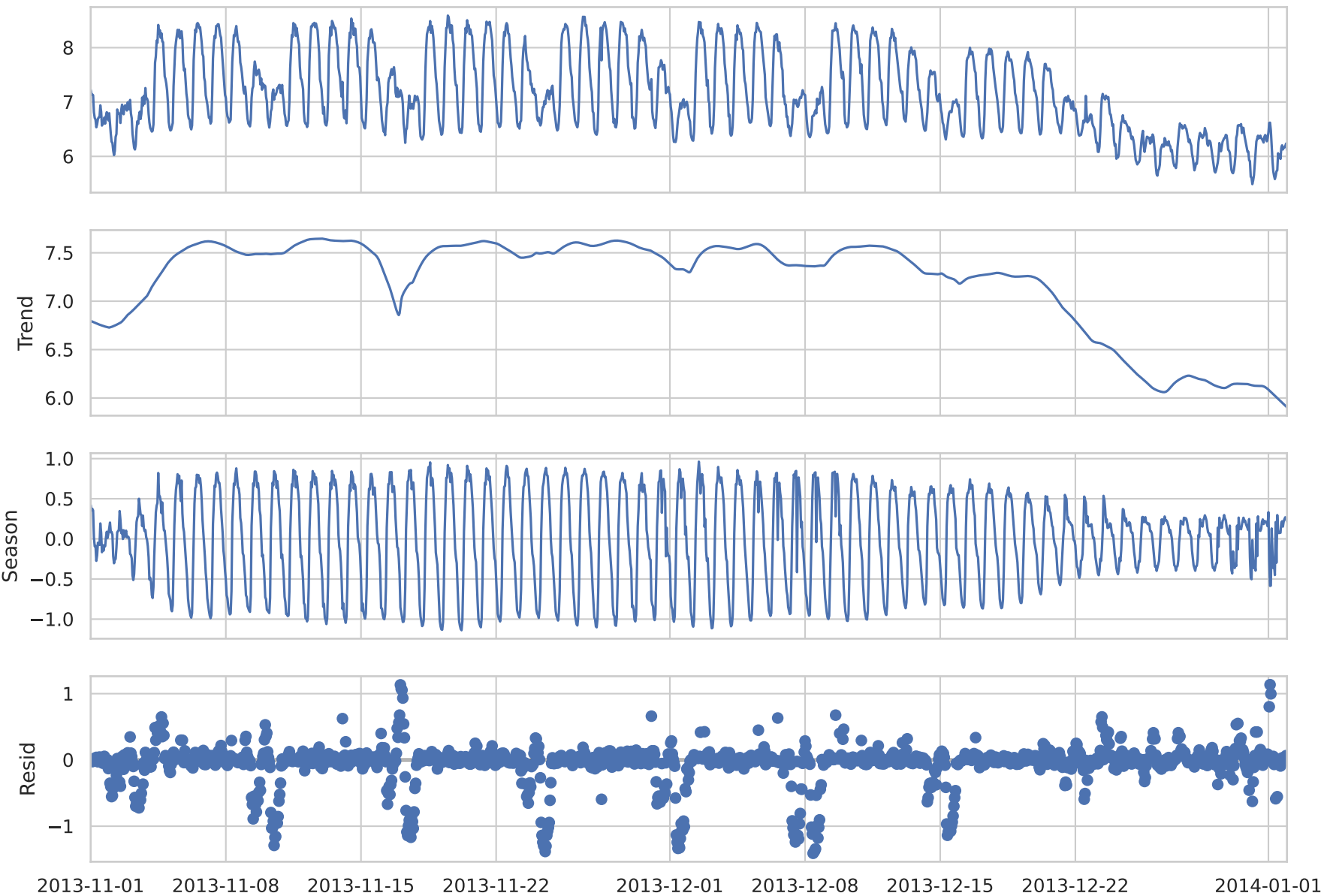
STL decomposition (period = 24 h) of \log(1+\text{bocconi})
